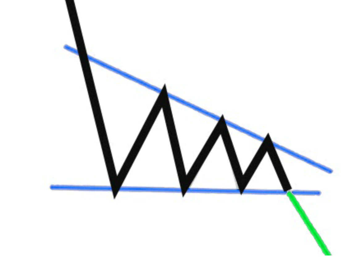
Ascending Triangle
