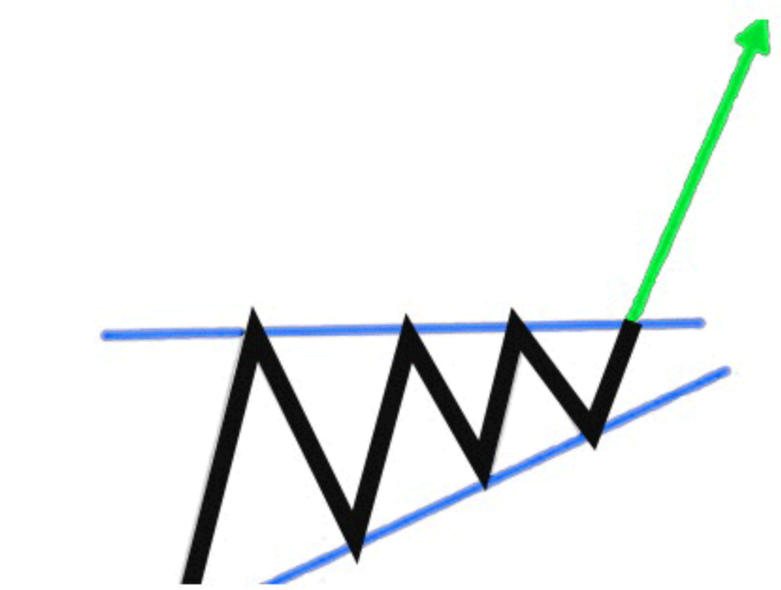
Descending Triangle
